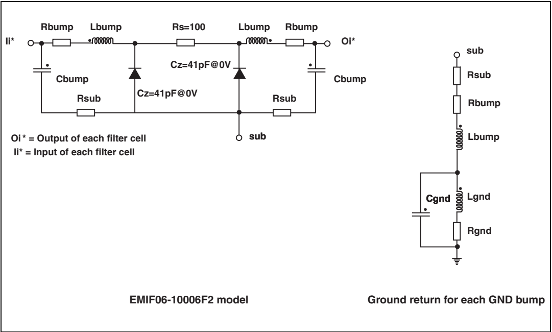
Figure 9. Aplac model
